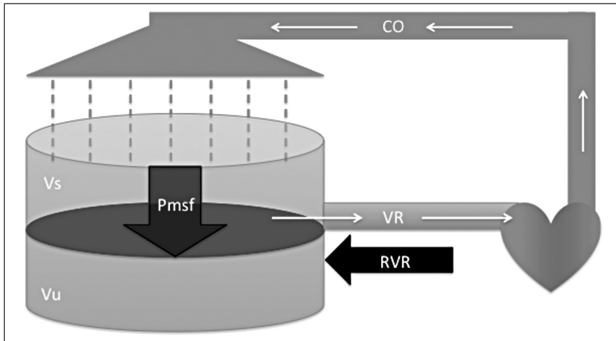
Figure 1. Schematic diagram of the cardiovascular system and the venous return. CO — cardiac output; Pmsf — mean systemic filling pressure; RVR — resistance to venous return; VR — venous return; Vs — stressed volume; Vu — unstressed volume
